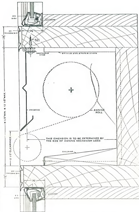
RECESSED AWNING BAR No. 958
